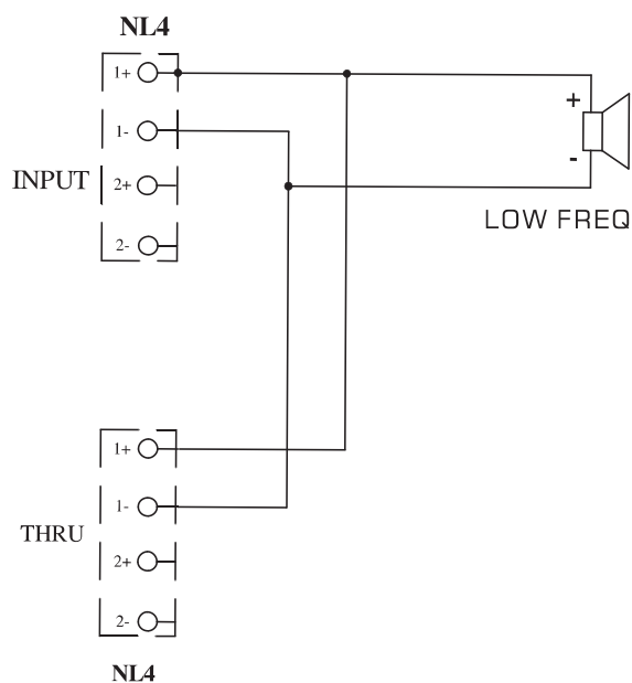
L-ARRAY 18S Block Diagram
